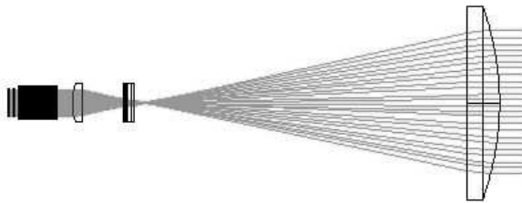
Figure 1: Side view of optical system
