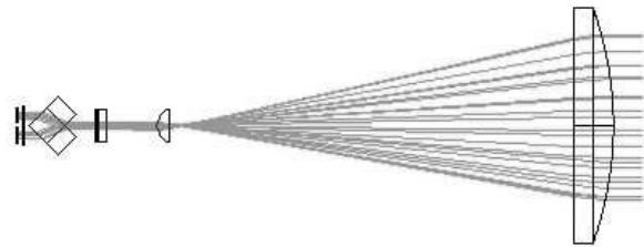
Figure 2: Top view of optical system
